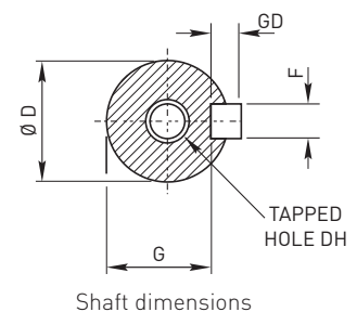
Shaft dimensions
